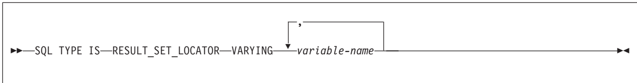
Figure 96. Result set locators
