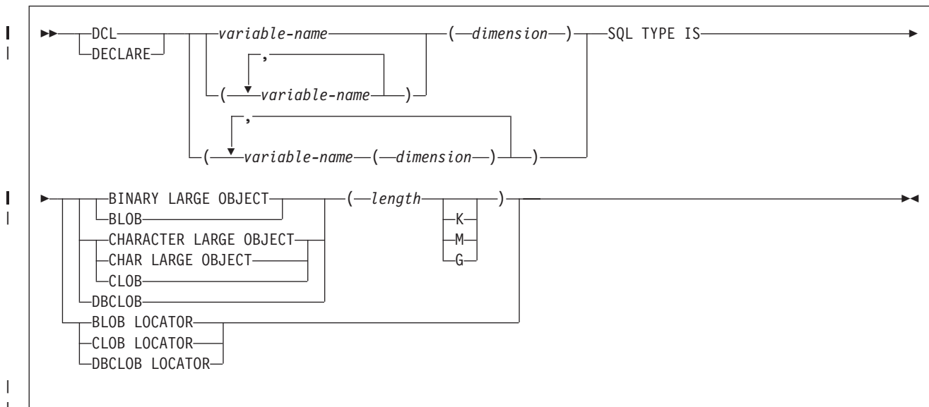
Figure 110. LOB variable arrays and locators
