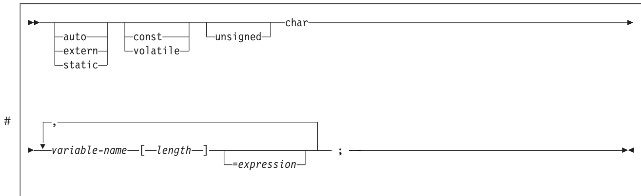
Figure 43. NUL-terminated character form
