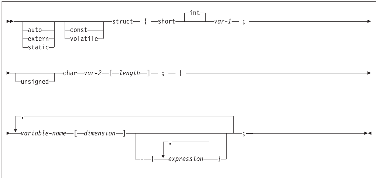
Figure 54. VARCHAR structured form
