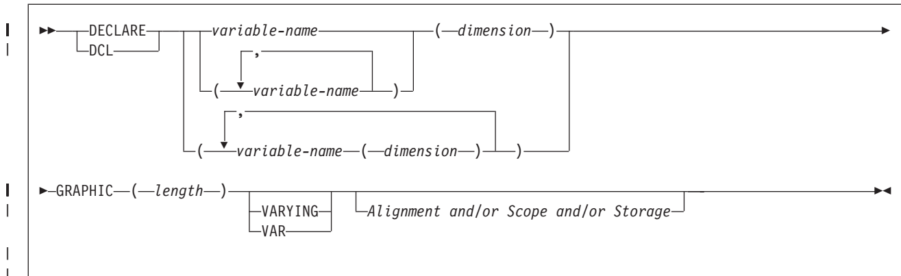
Figure 109. Graphic host variable arrays
