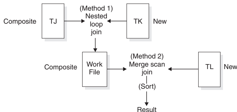
Figure 231. Two-step join operation
