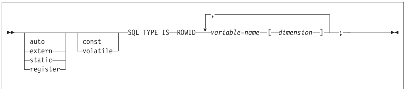
Figure 58. ROWID variable arrays
