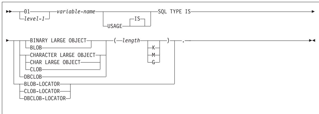
Figure 74. LOB variables and locators
