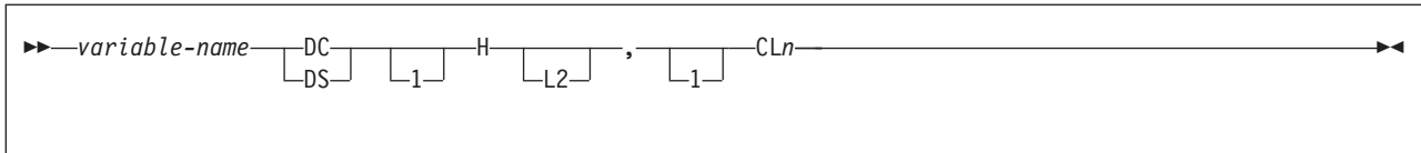
Figure 33. Varying-length character strings
