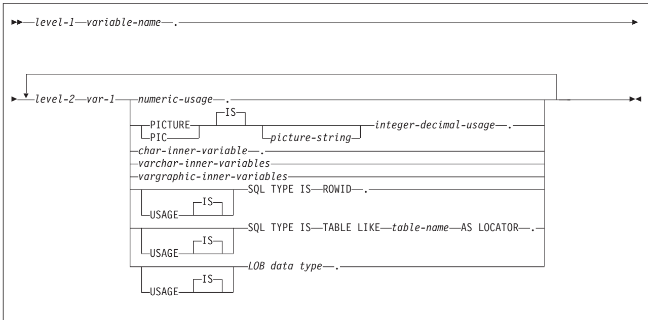
Figure 85. Host structures in COBOL
