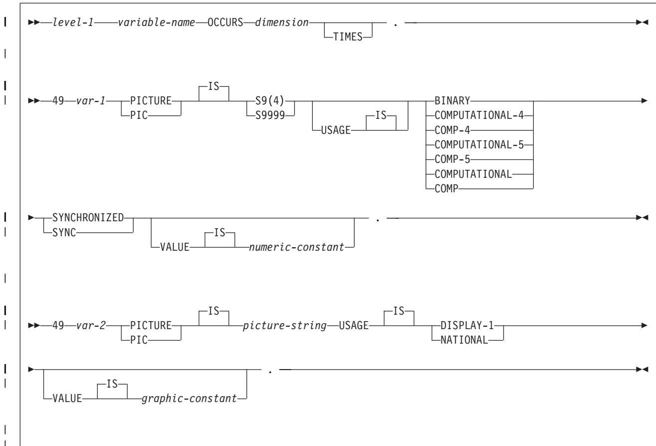
Figure 82. Varying-length graphic string arrays
