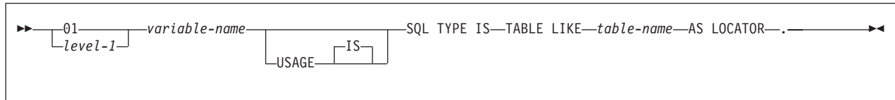
Figure 73. Table locators
