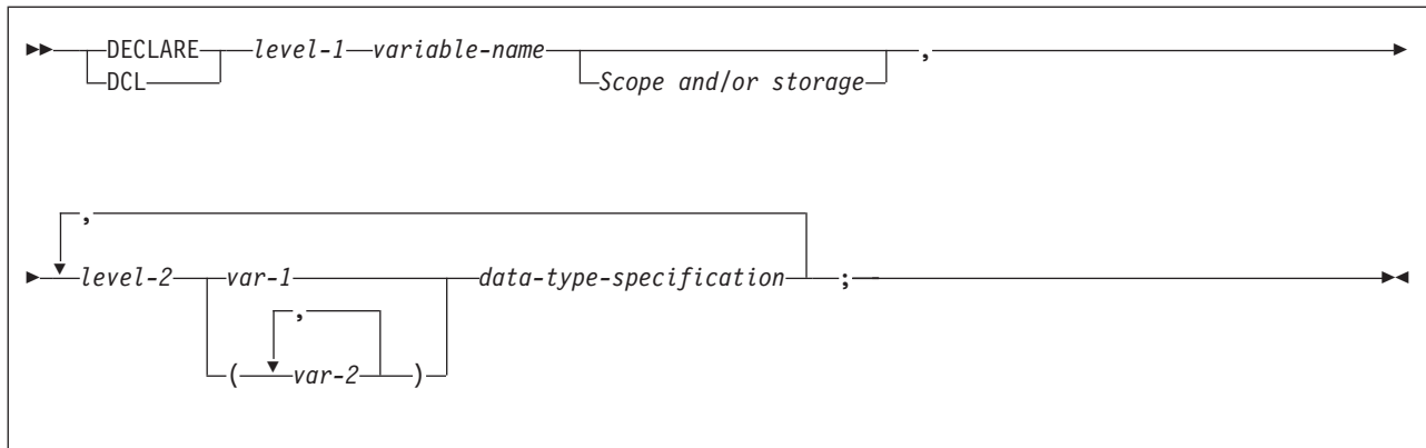
Figure 112. Host structures
