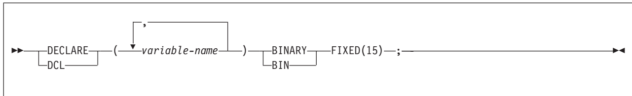
Figure 115. Indicator variable
