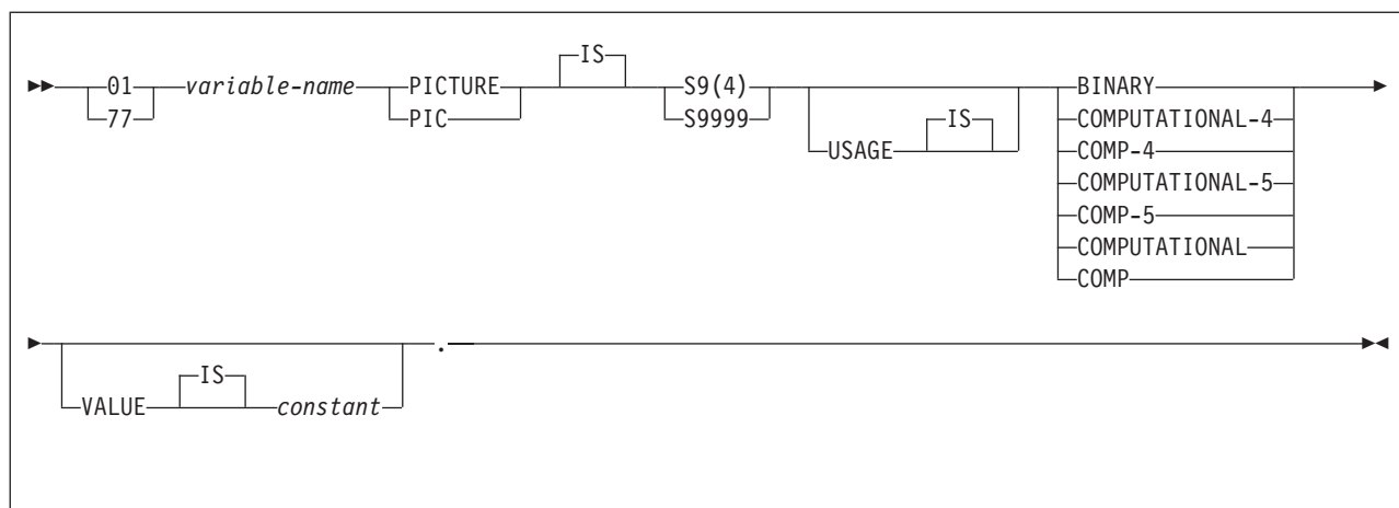
Figure 92. Indicator variable
