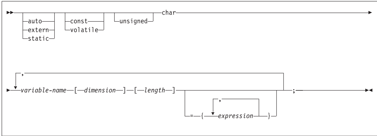
Figure 53. NUL-terminated character form
