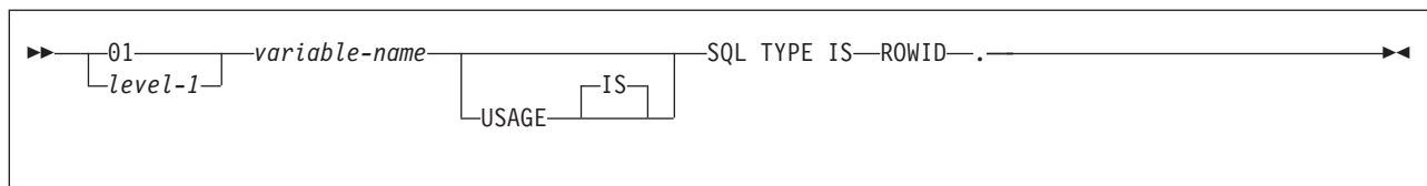
Figure 75. ROWID variables
