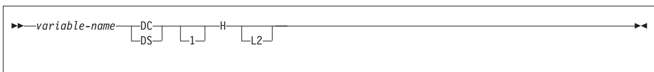
Figure 40. Indicator variable
