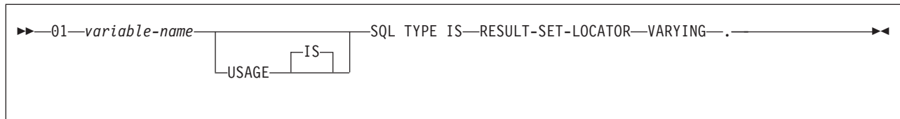
Figure 72. Result set locators
