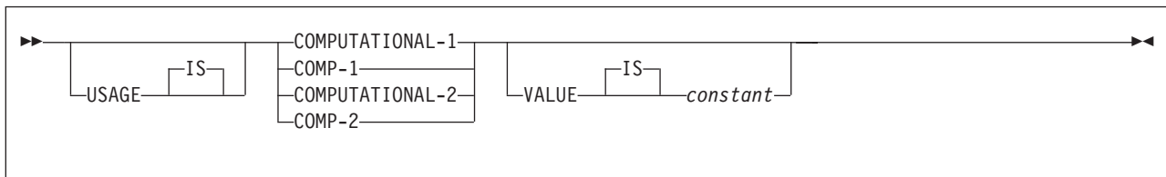
Figure 86. Numeric-usage
