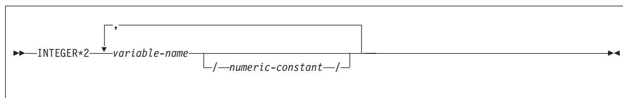
Figure 99. Indicator variable
