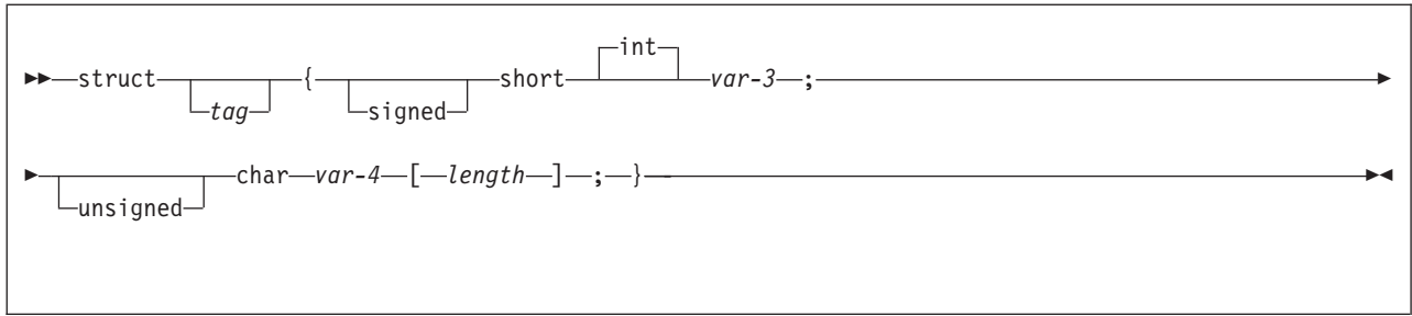
Figure 60. VARCHAR-structure
