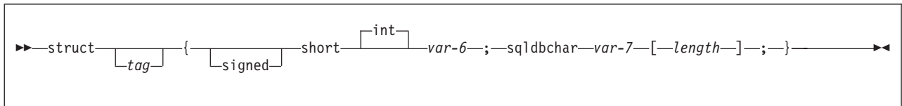
Figure 61. VARGRAPHIC-structure
