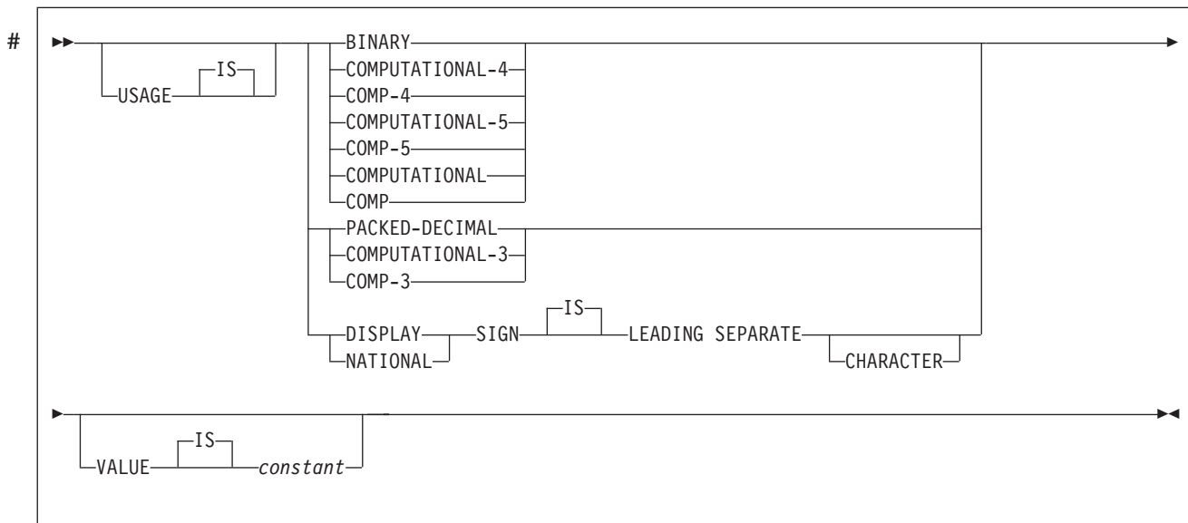
Figure 87. Integer-decimal-usage
