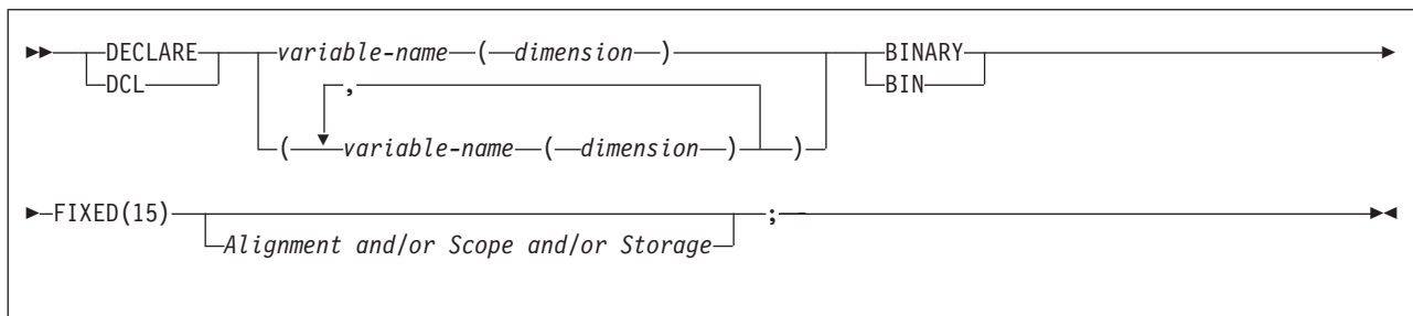
Figure 116. Indicator array
