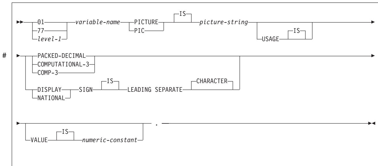
Figure 67. Decimal host variables
