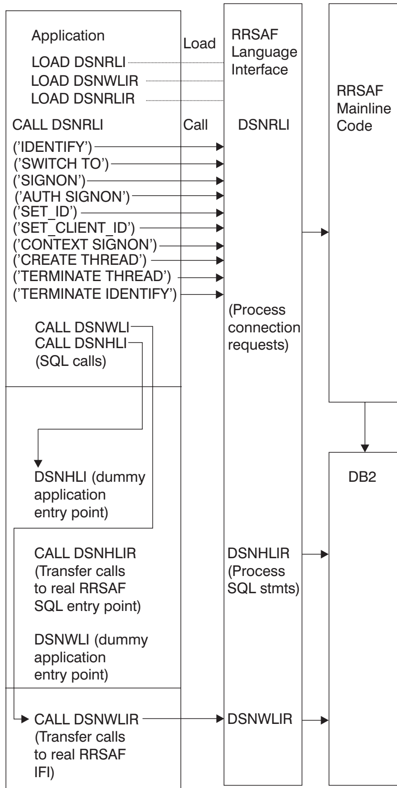
Figure 247. Sample RRSAF configuration
