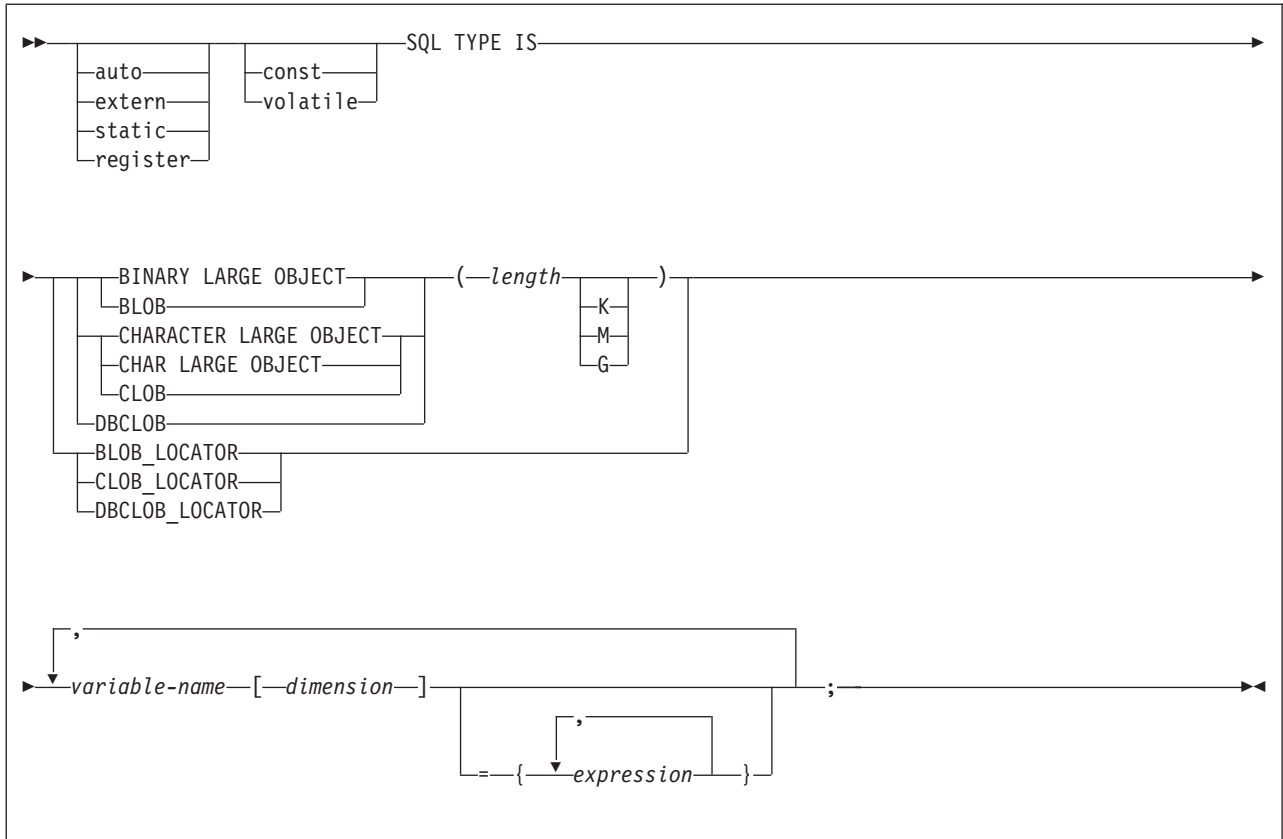
Figure 57. LOB variable arrays and locators
