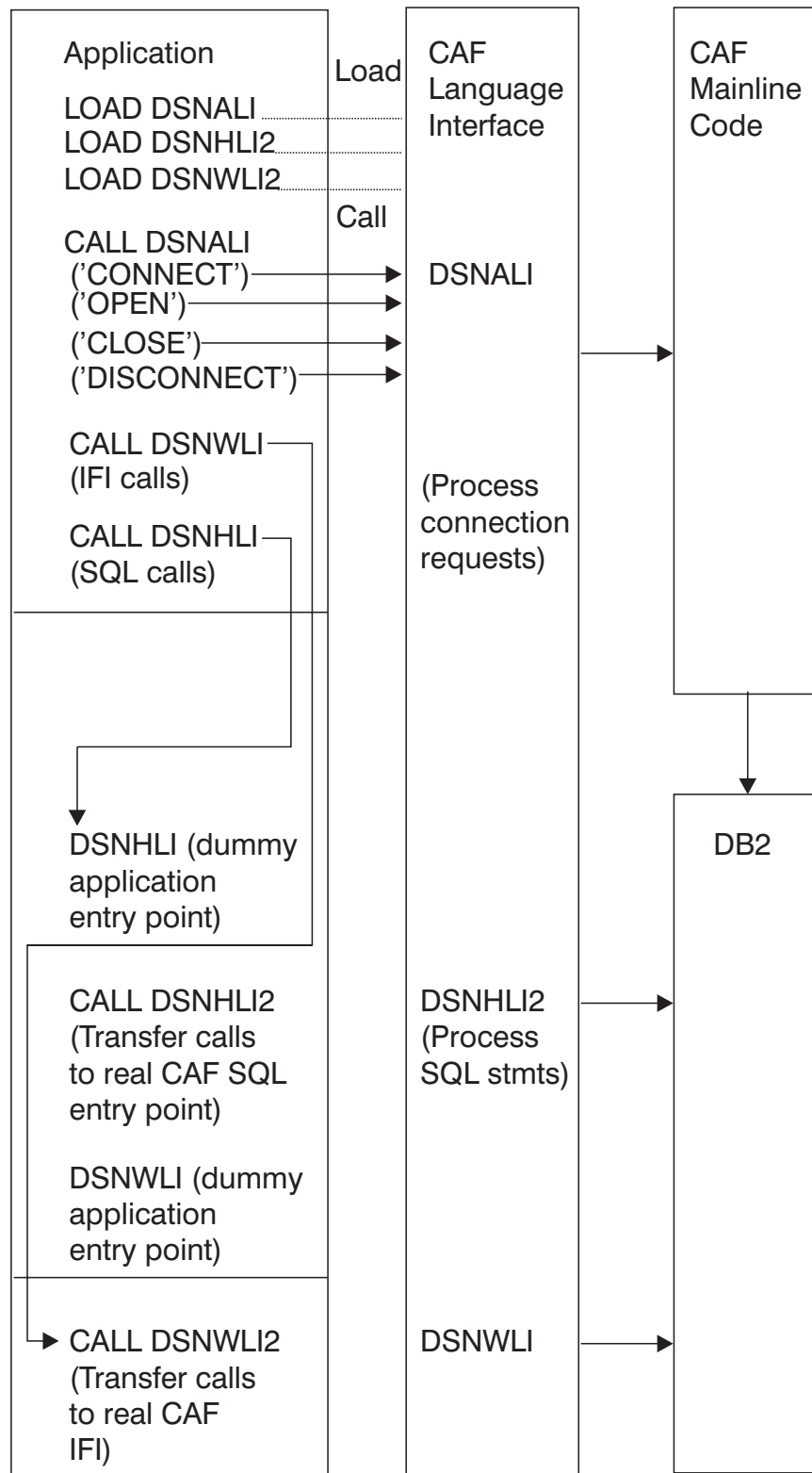
Figure 242. Sample call attachment facility configuration
