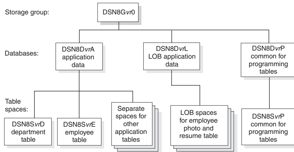
Figure 270. Relationship among sample databases and table spaces
