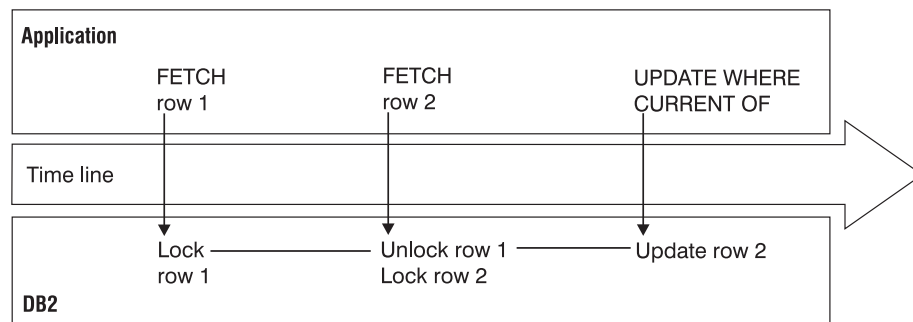
Figure 143. Positioned updates and deletes with a static non-scrollable cursor and without optimistic concurrency control
