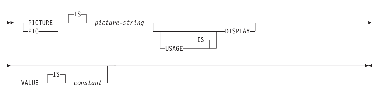
Figure 88. CHAR-inner-variable
