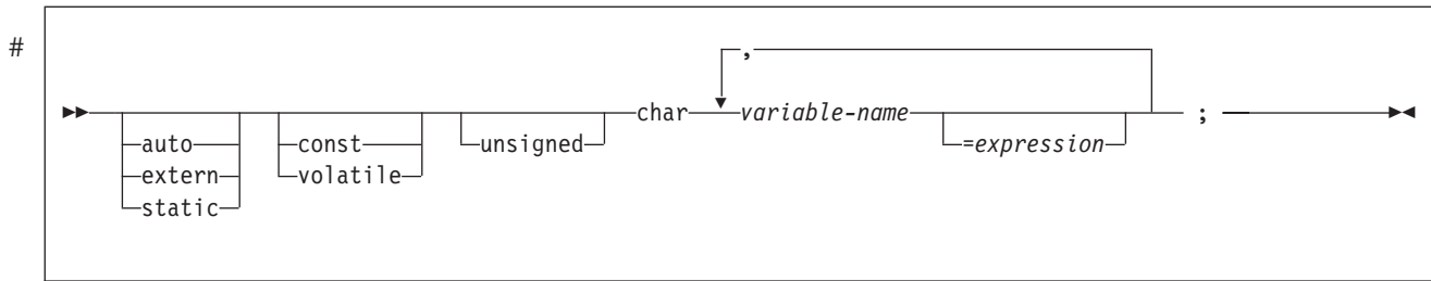
Figure 42. Single-character form
