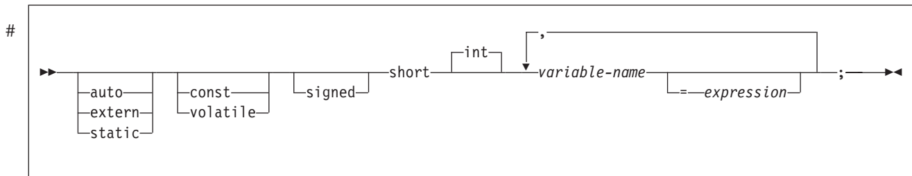
Figure 63. Indicator variable
