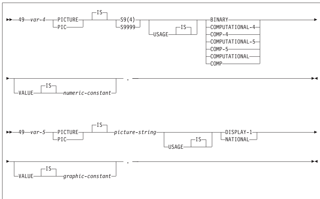
Figure 90. VARGRAPHIC-inner-variables
