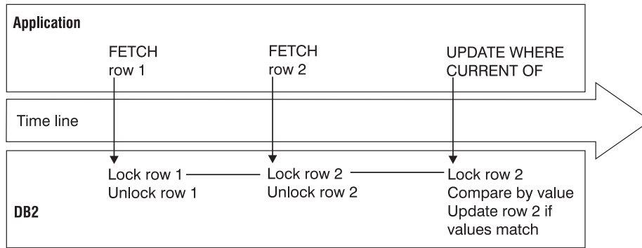
Figure 144. Positioned updates and deletes with a static sensitive scrollable cursor and with optimistic concurrency control
