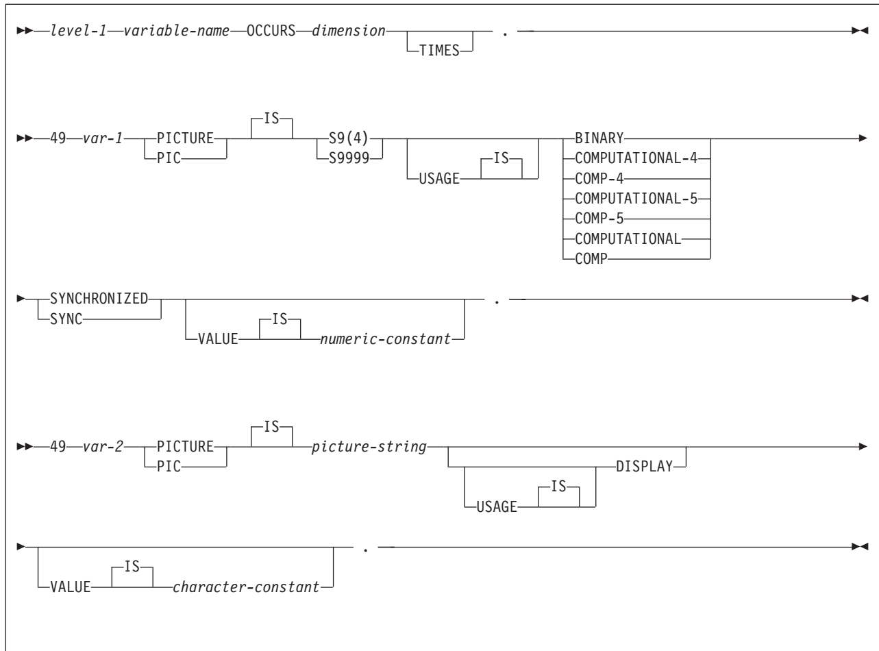
Figure 80. Varying-length character string arrays
