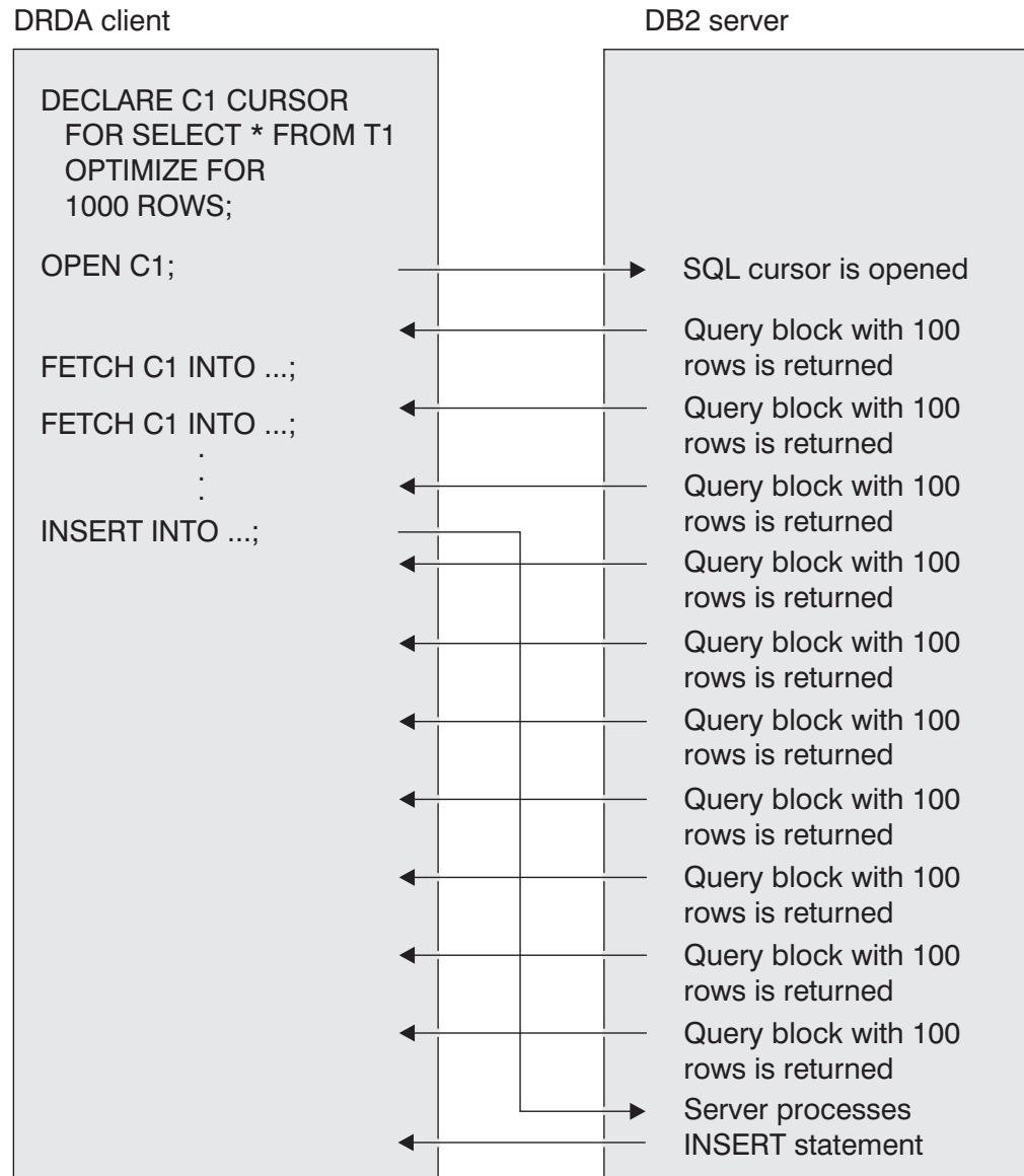
Figure 150. Message flows with OPTIMIZE FOR 1000 ROWS
